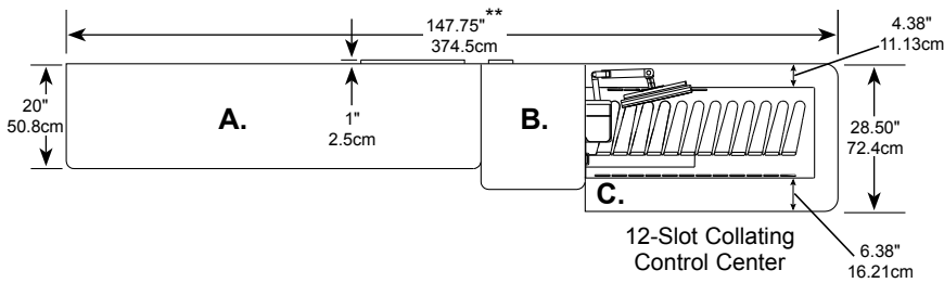
Front View
